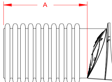
SC-740 - 24" PIPE SC740EPE24BL
